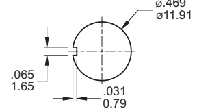
15/32IN BUSHING
