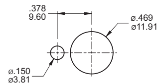
15/32IN BUSHING
