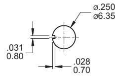
METRIC BUSHING
