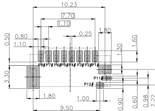
RECOMMENDED PCB LAYOUT TOL:(±0.05)
