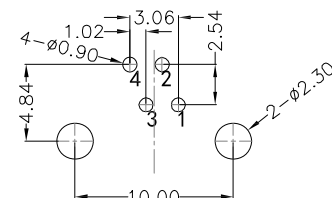
RECOMMENDED PCB LAYOUT VIEWED FROM COMPONENT SIDE
