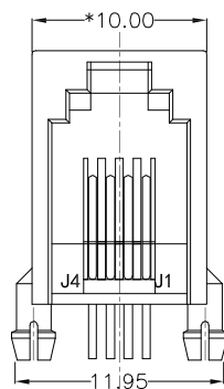
FRONT VIEW
