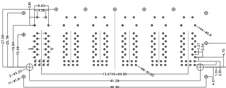
RECOMMENDED PCB LAYOUT VIEWED FROM COMPONENT SIDE
