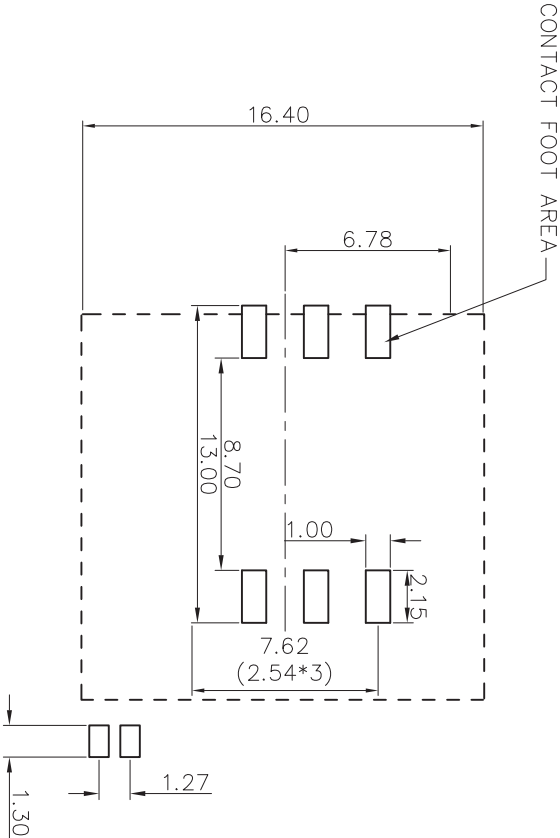
REFERENCE PC BOARD LAYOUT
