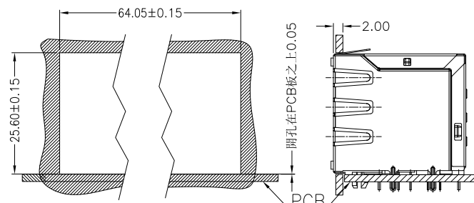
RECOMMENDED PANEL CUTOUT DIMENSION
