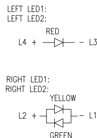
LED SCHEMATIC:
