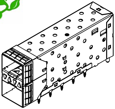
(4 LIGHT PIPE) E90-K110-4004
