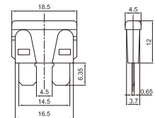
ATQ FUSE
